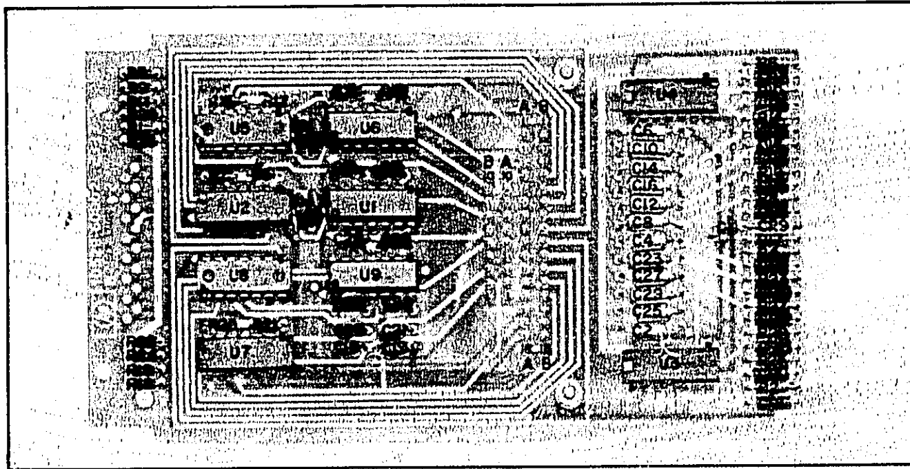
Figure 8-3. Main Beard Component Locations
