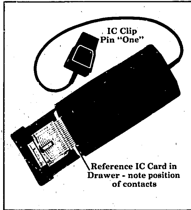
Figure 3-3. Reference IC Card in Comparator Drawer
