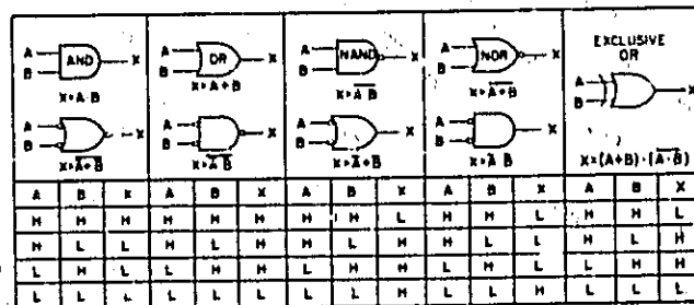
Figure 4-1. Gate Symbols and Logic Comparisons
