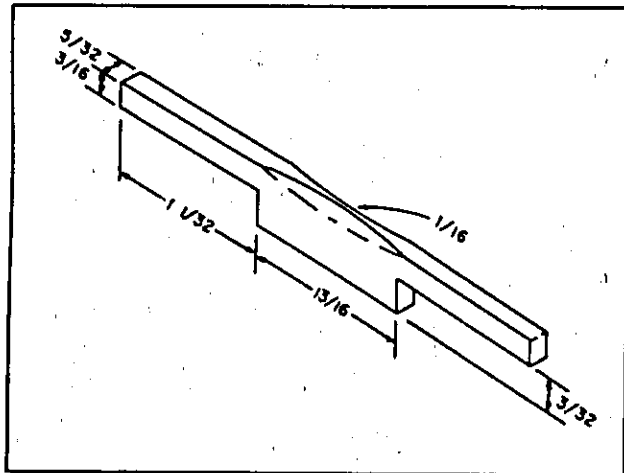
Figure 5-6. Extractor Tool
